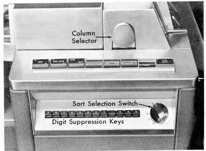
Figure 16. Machine Controls (83)
