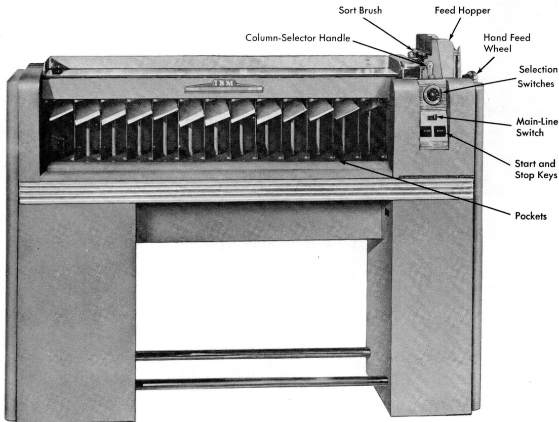
Figure 2. IBM 82 Sorter
