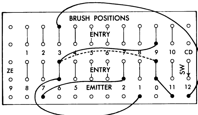
Figure 43. Selection of Alpha-Numerical Punching (83)
