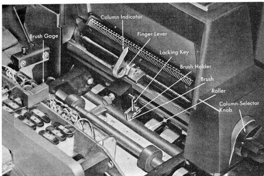
Figure 18. Sort-Brush Assembly (83)
