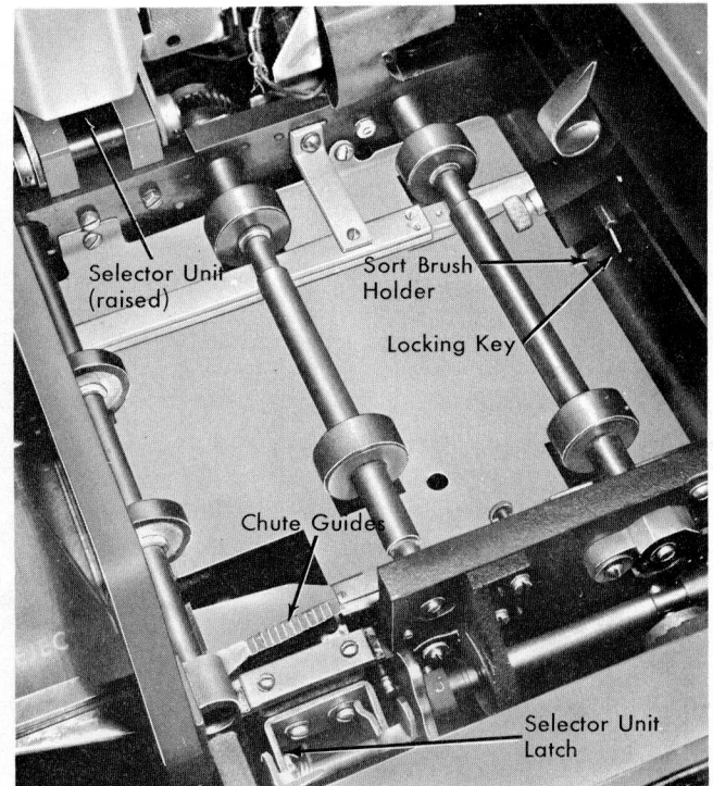
Figure 22. Selector Assembly and Latch (83)
