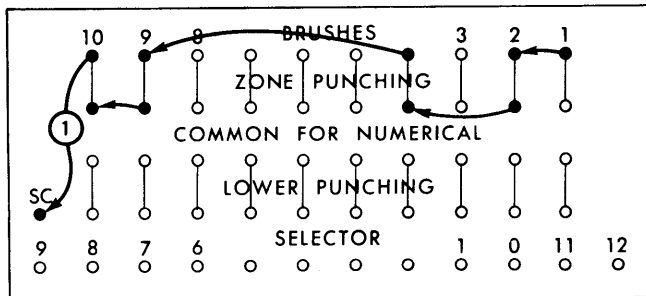
Figure 37. Common-Digit Selection (82)
