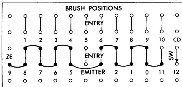
Figure 46. Zero Elimination (83)
