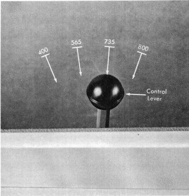
Figure 20. Control Lever for Adjusting Pocket Stop (83)
