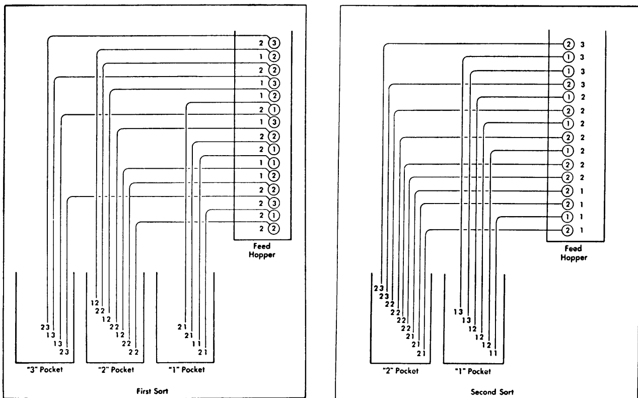
Figure 7. Sorting Principle
