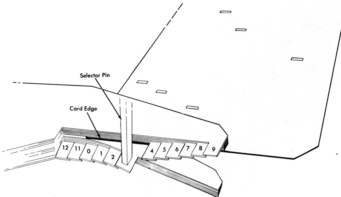
Figure 21. Chute Blades (83)
