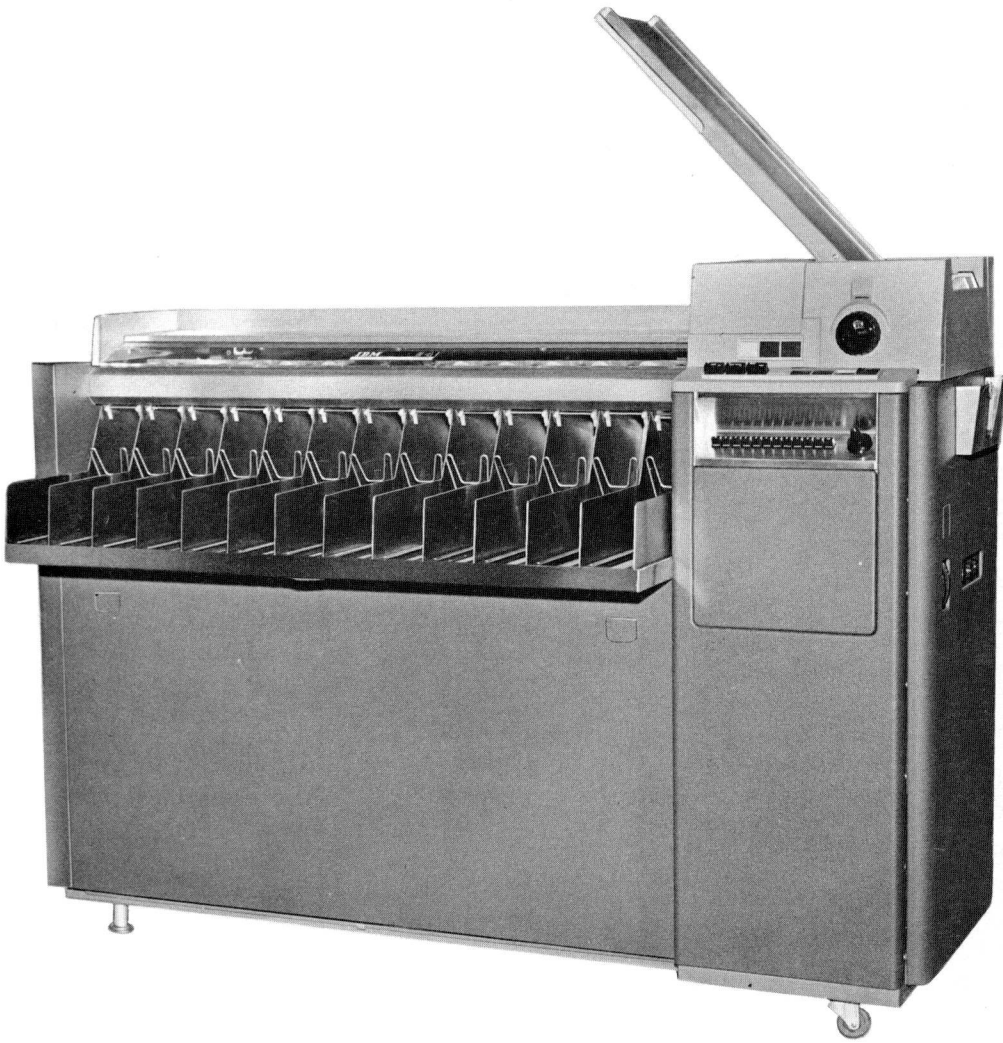
Figure 1. IBM 84 Sorter
