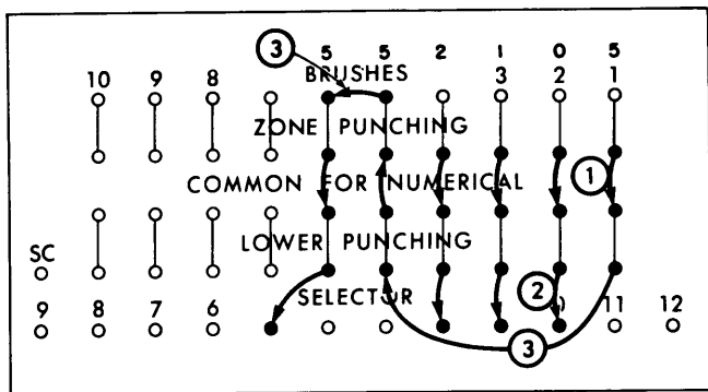
Figure 40. Multiple-Column Selection of Numerical Information (82)
