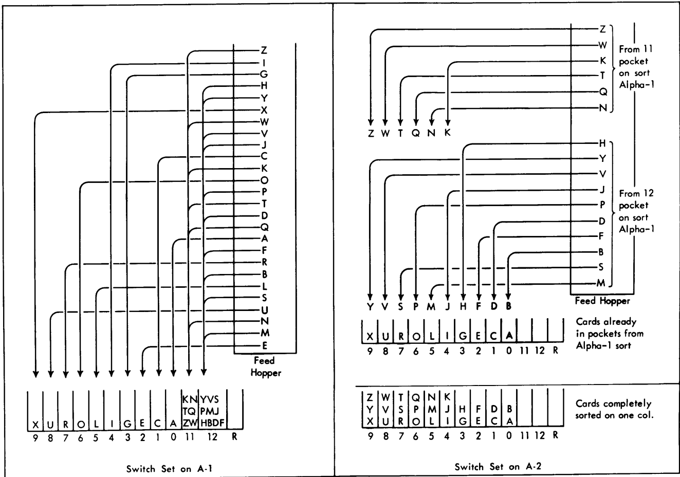
Figure 30. Sorting Principle Using Alphabetic Sorting Feature
