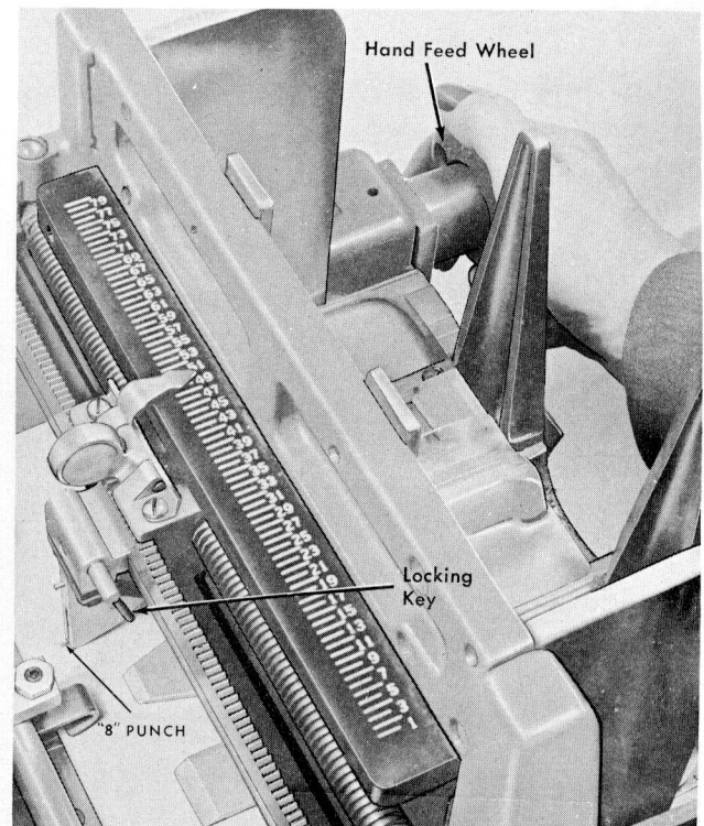
Figure 11. Timing the Brush (82)
