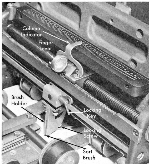
Figure 4. Sort Brush and Column Indicator (82)
