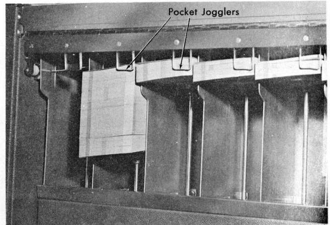
Figure 34. Pocket Jogglers
