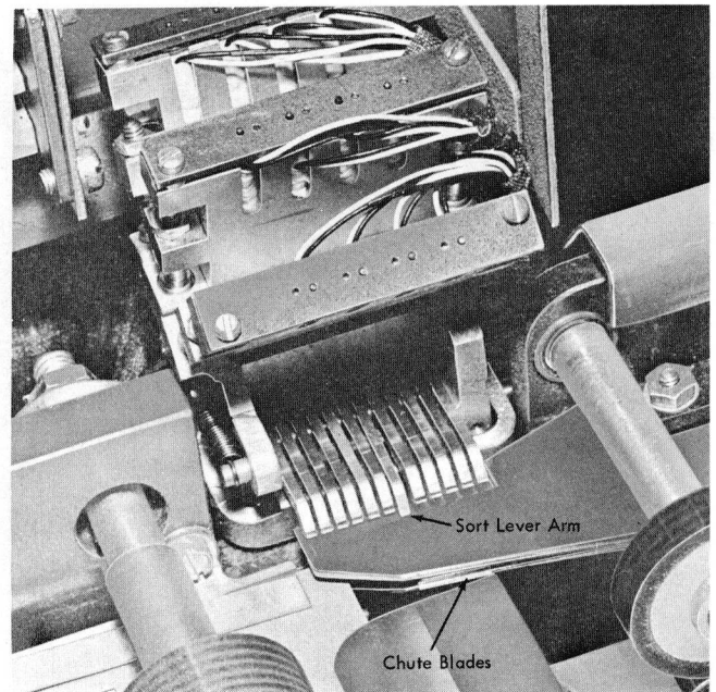
Figure 26. Selector Unit
