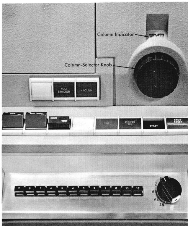
Figure 23. Machine Controls (84)
