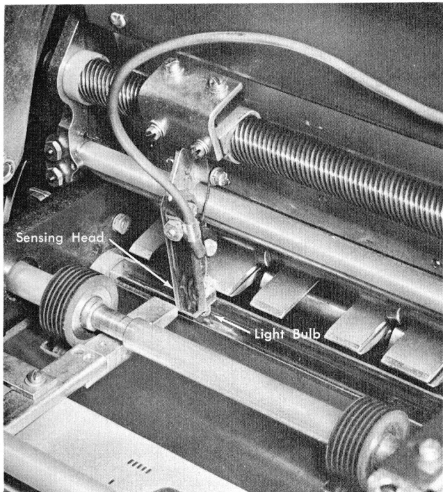
Figure 25. Sensing Mechanism (84)
