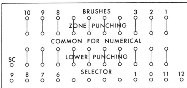
Figure 36. Multiple-Column Selection Feature Control Panel (82)
