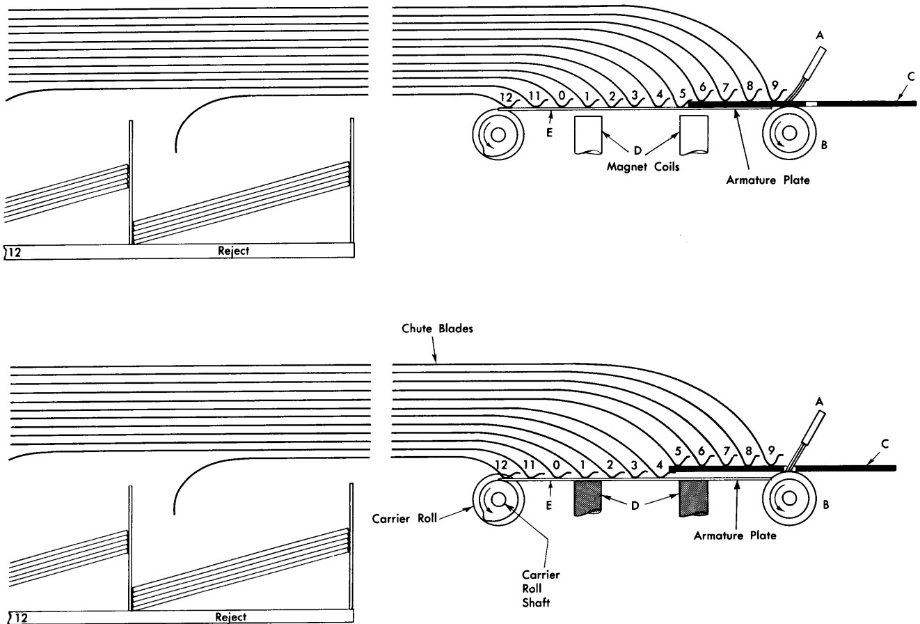
Figure 6. Schematic of Card Feed (82)
