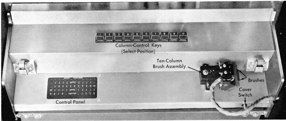
Figure 35. Ten-Column Brush Assembly, Control Panel, Keys, and Switches on the IBM 83 Sorter
