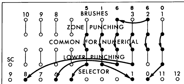
Figure 42. Multiple-Column Selection with Normal Sorting (82)
