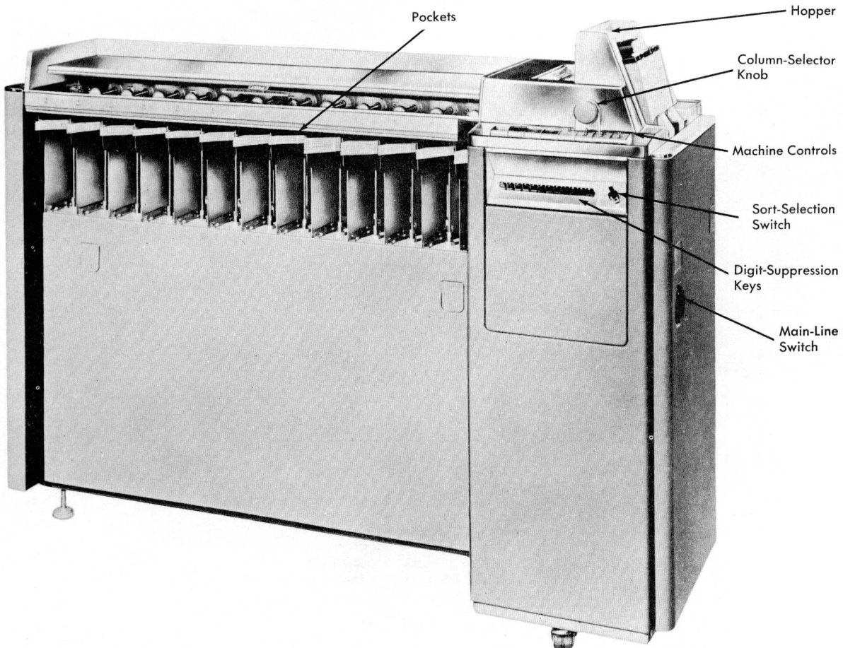
Figure 15. IBM 83 Sorter
