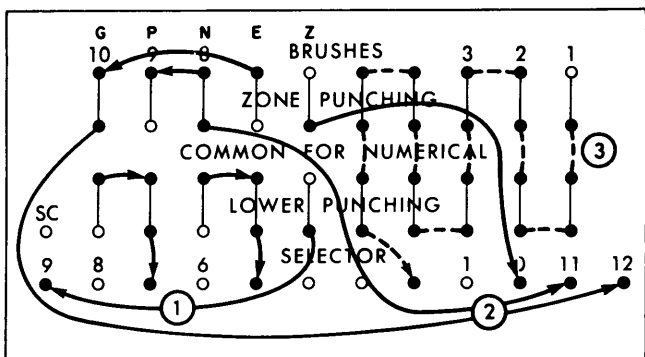
Figure 41. Multiple-Column Selection of Alphabetic Information (82)
